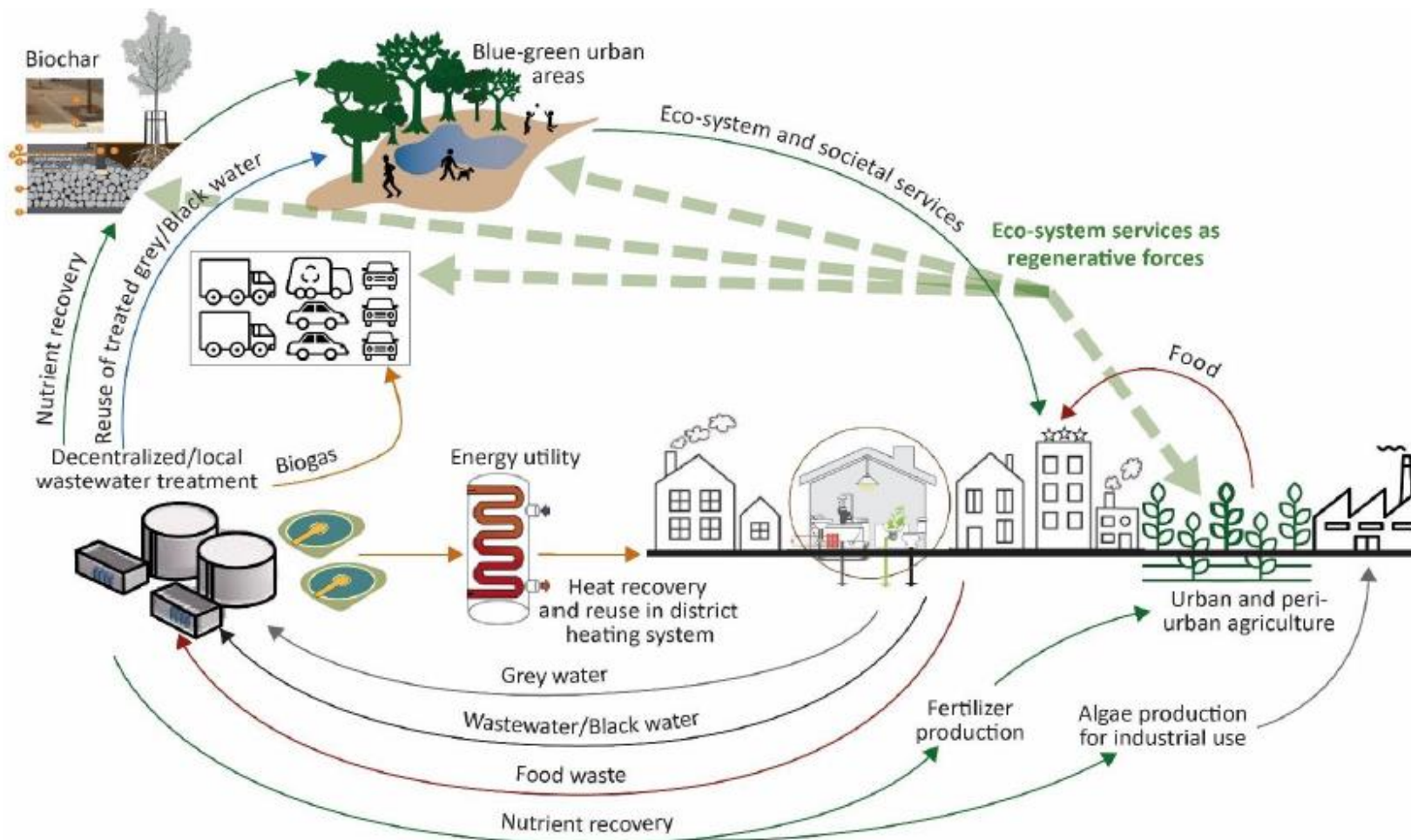
Figure 8: Circular sanitation in Stockholm
